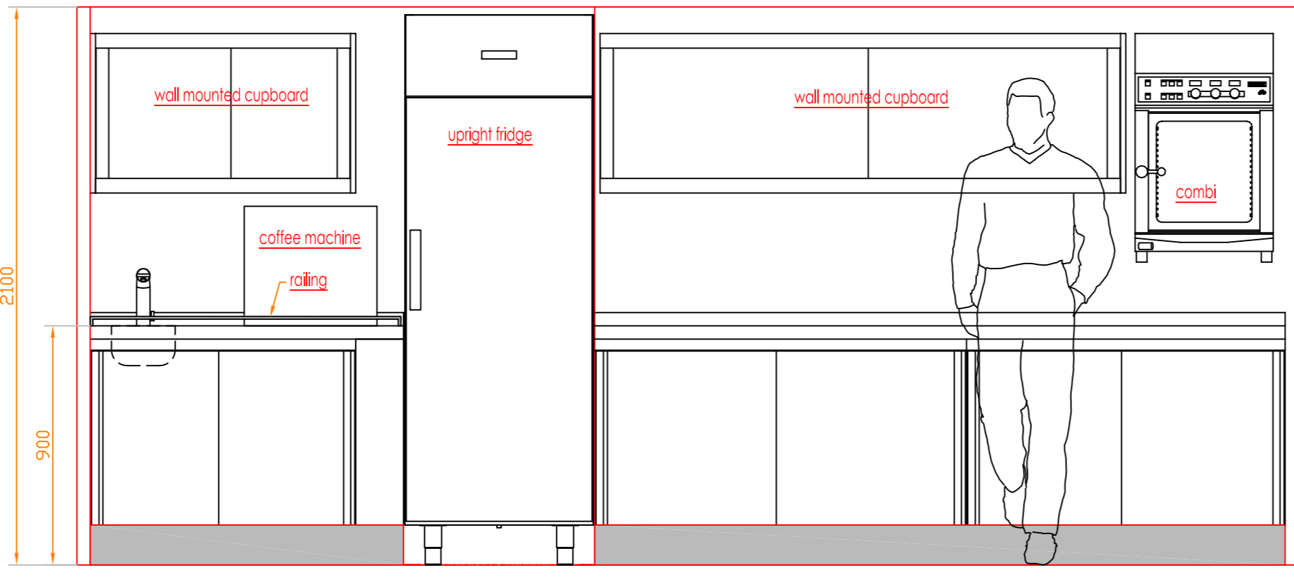
front view coffee-station - combi steamer
